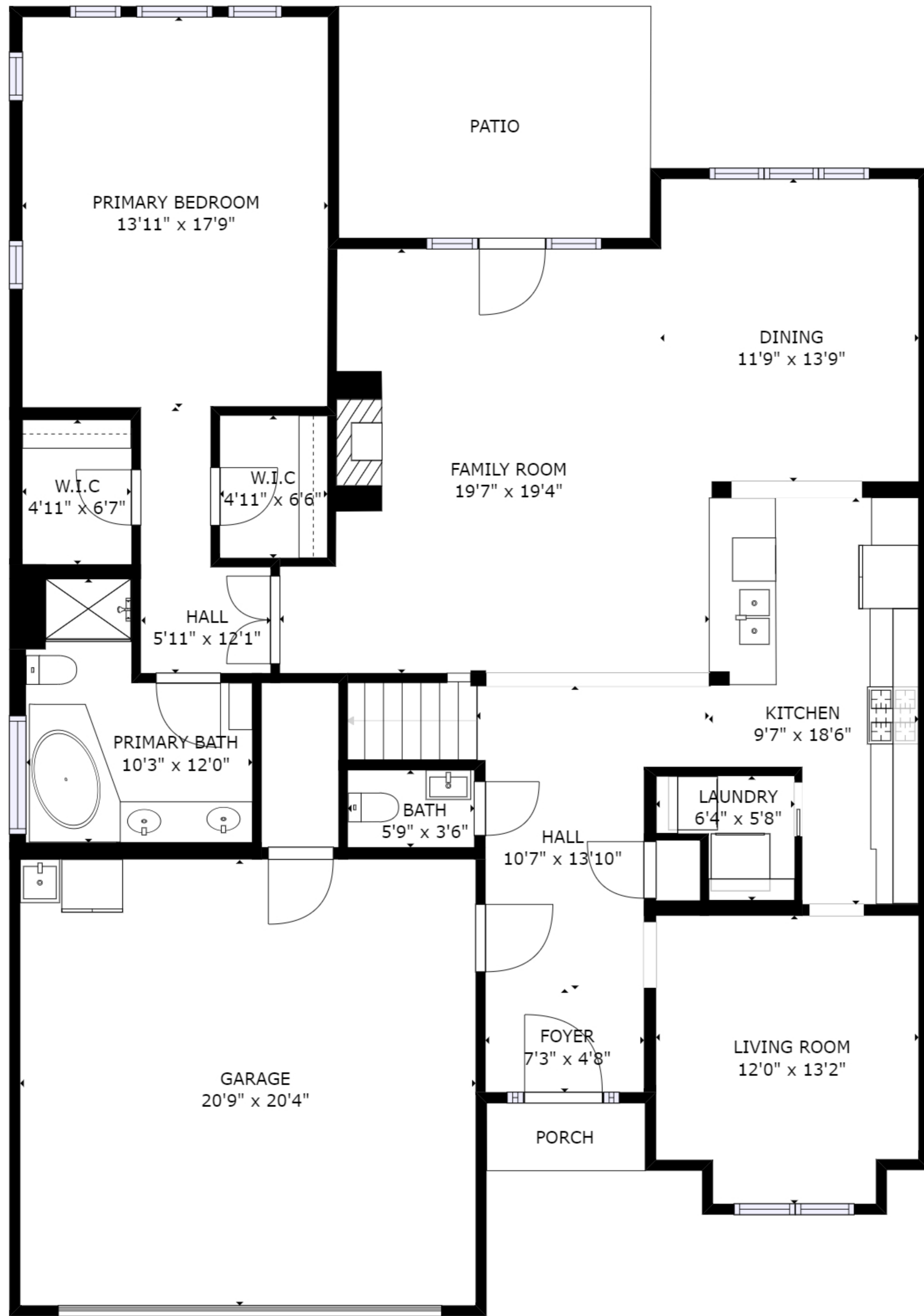
FLOOR 1
